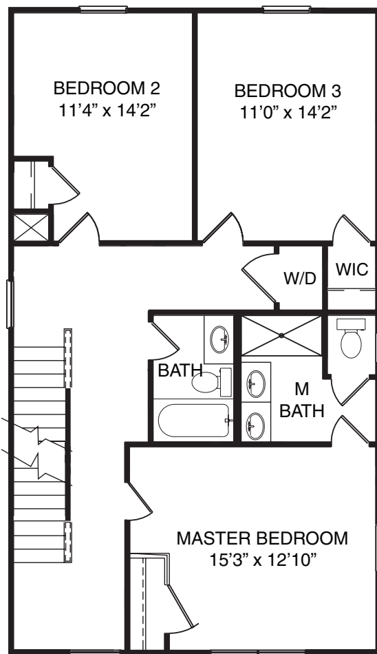
OPT. SECOND FLOOR
